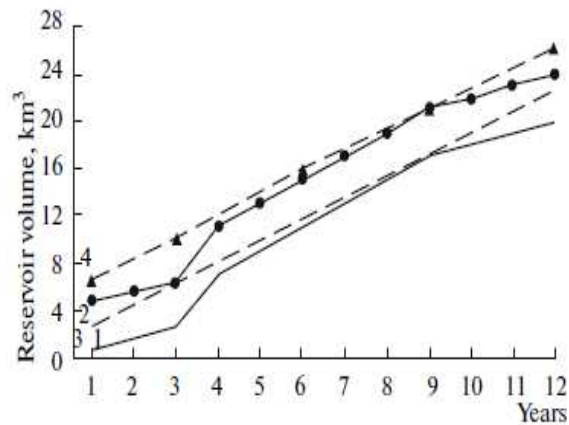
Figure 1. Multipurpose runoff regulation by two reservoirs. 1,2-filled and emptied state of the reservoir, respectively, 3,4-the regime of hydropower regulation at the filled and emptied state of two reservoir, respectively.
