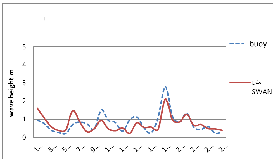
Figure 4. Comparing buoy data and SWAN output april 2011
