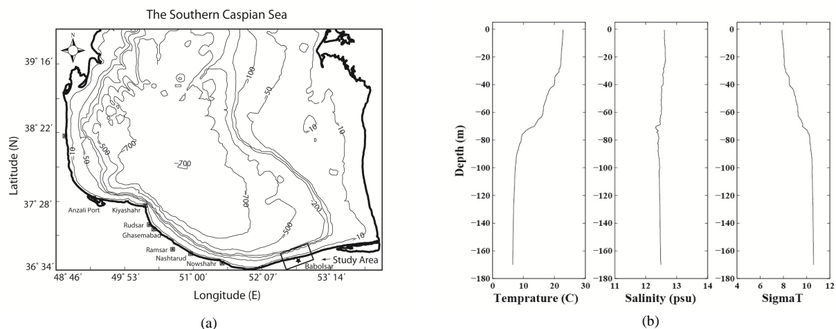
Figure 1: a) The southern Caspian basin, b) Vertical profiles of temperature, salinity and density
